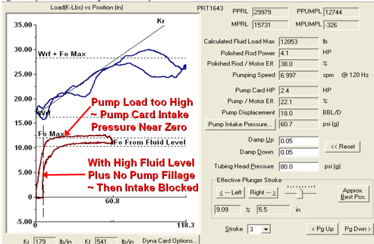
Figure 2 – Dynamometer Card Acquired Immediately After Well Down for 10 Minutes
