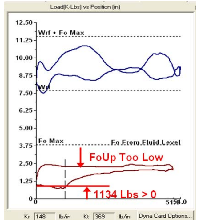
Figure 4 – Initial dynamometer card on the Well
