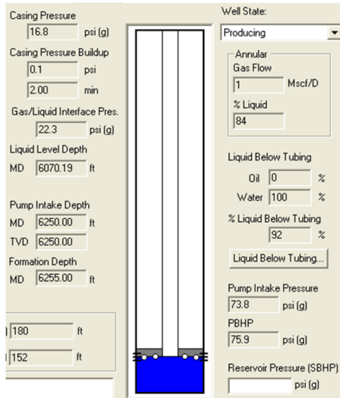
Figure 5 – Fluid Level on Well 3 Shot Down the Tubing/Casing Annulus
