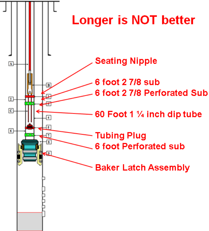
Figure 4 – Poor Boy Down Hole Gas Separator with 60 Foot Dip Tube
