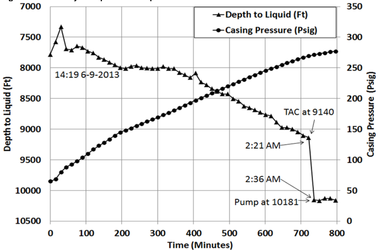
Figure 9 – Summary of Liquid Level Depression Test
