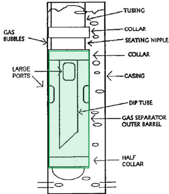
Figure 2 – Collar Sized Gas Separator
