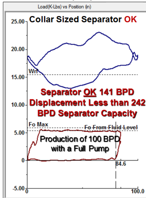
Figure 3 – Example of Gas Separator Selection with Sufficient Capacity
