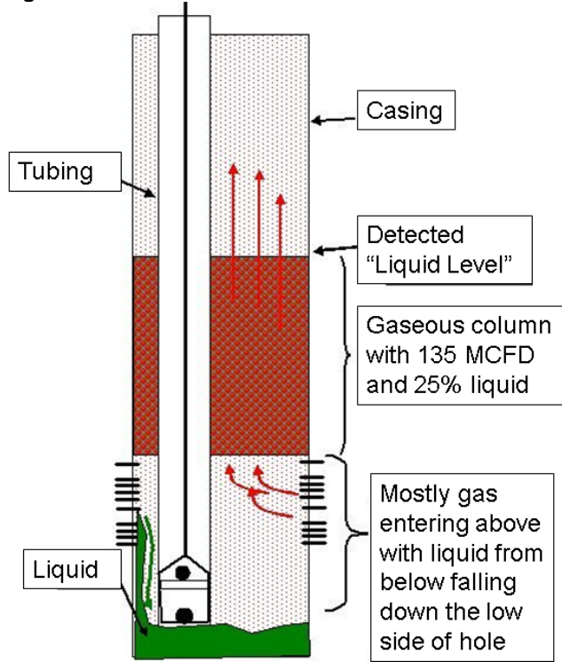
Figure 9 – Summary of Liquid Level Depression Test
