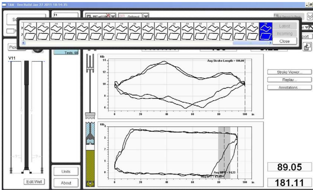
Figure 8 – Dynamometer Replay and Stroke Overlay.
