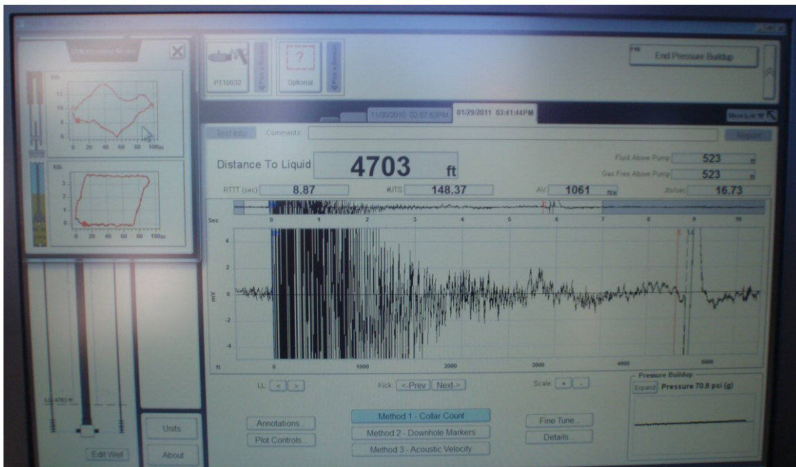
Figure 4 - Simultaneous Real-time Monitoring of Dynamometer and Acoustic Fluid Level Acquisition.
